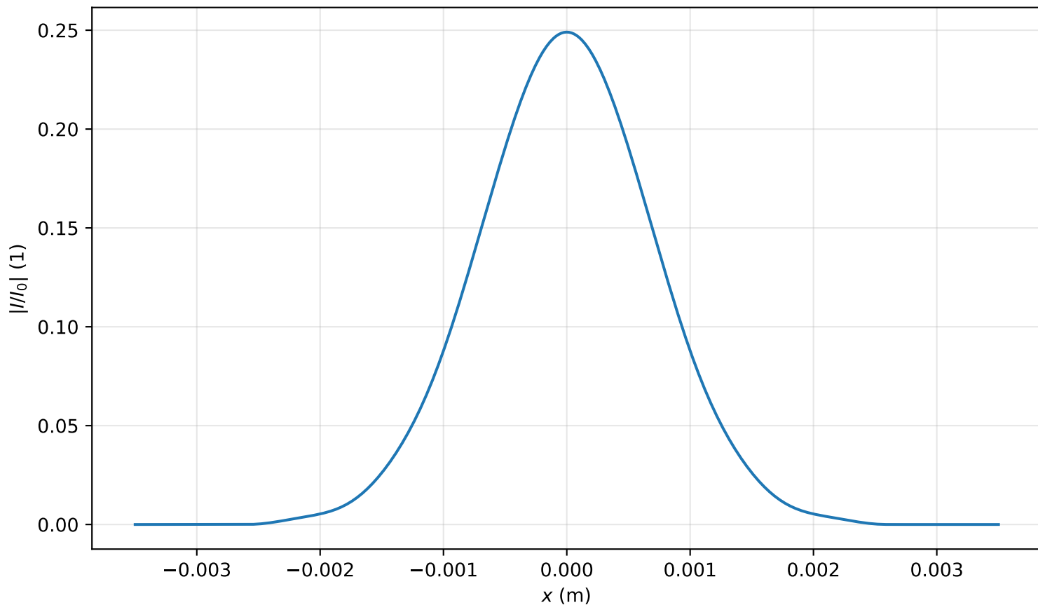
Intensity profile I(x, y = 0, z = 3.981m)/I_0 , P_{in}=0.2P_{cr} , artificial time
